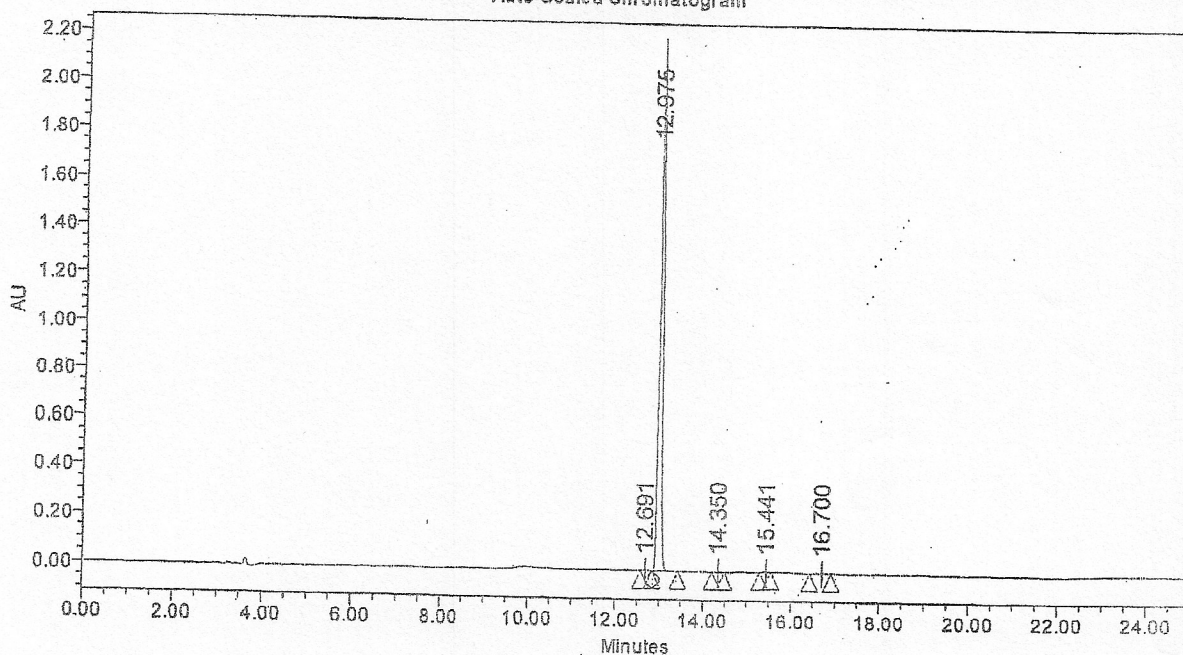
Auto-Scaled Chromatogram
